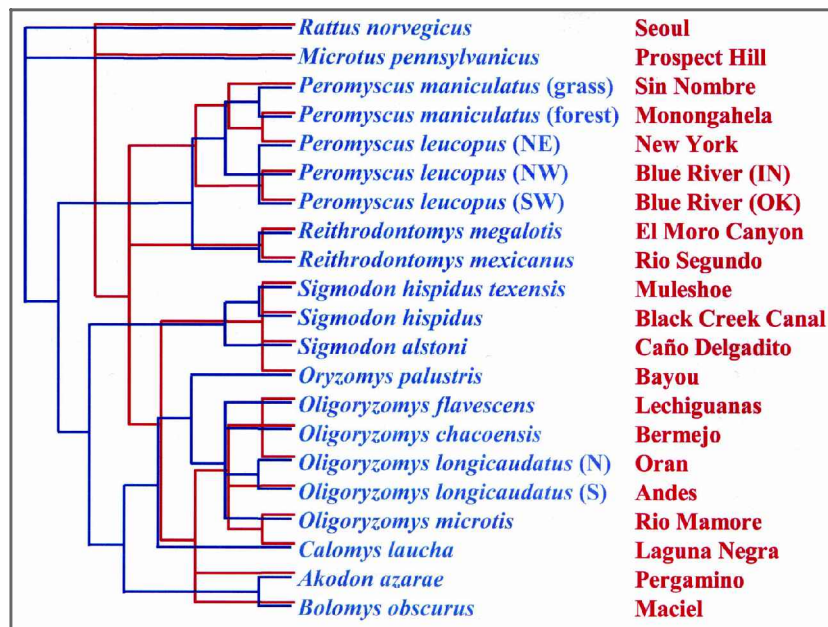
Figure 3. Phylogenetic relationships of hantaviruses (red) compared with their rodent hosts (blue). Virus phylogenies are based primarily on the M-segment genome but include some S-segment data as well. The rodent phylogeny is based on cytochrome b mitochondrial DNA sequence. The virus phylogeny was obtained from Plyushin and Morzunov (2001) and citations therein. The rodent phylogeny was obtained from Smith and Patton (1999).
